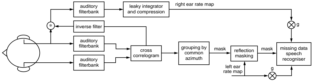
Figure 1: Schematic diagram of the right ear of the model.
